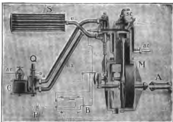
FIG. 281.—Diagram showing the Essential Features of a Typical Carriage Motor, as used on the De Dion Vehicles. M is the motor; C, the carburetter; S, the muffer; P, the sparking battery; B, the induction coil and condenser; Q, the pipe admitting pure air into muffer; aa, pipe for bringing hot air from around exhaust pipe; e, exhaust into muffer; a, pipe admitting gas to cylinder; ac, gasoline feed to carburetter; ac, port for admitting water to the jacket space of the cylinder; sc, exit port from the water jacket.
